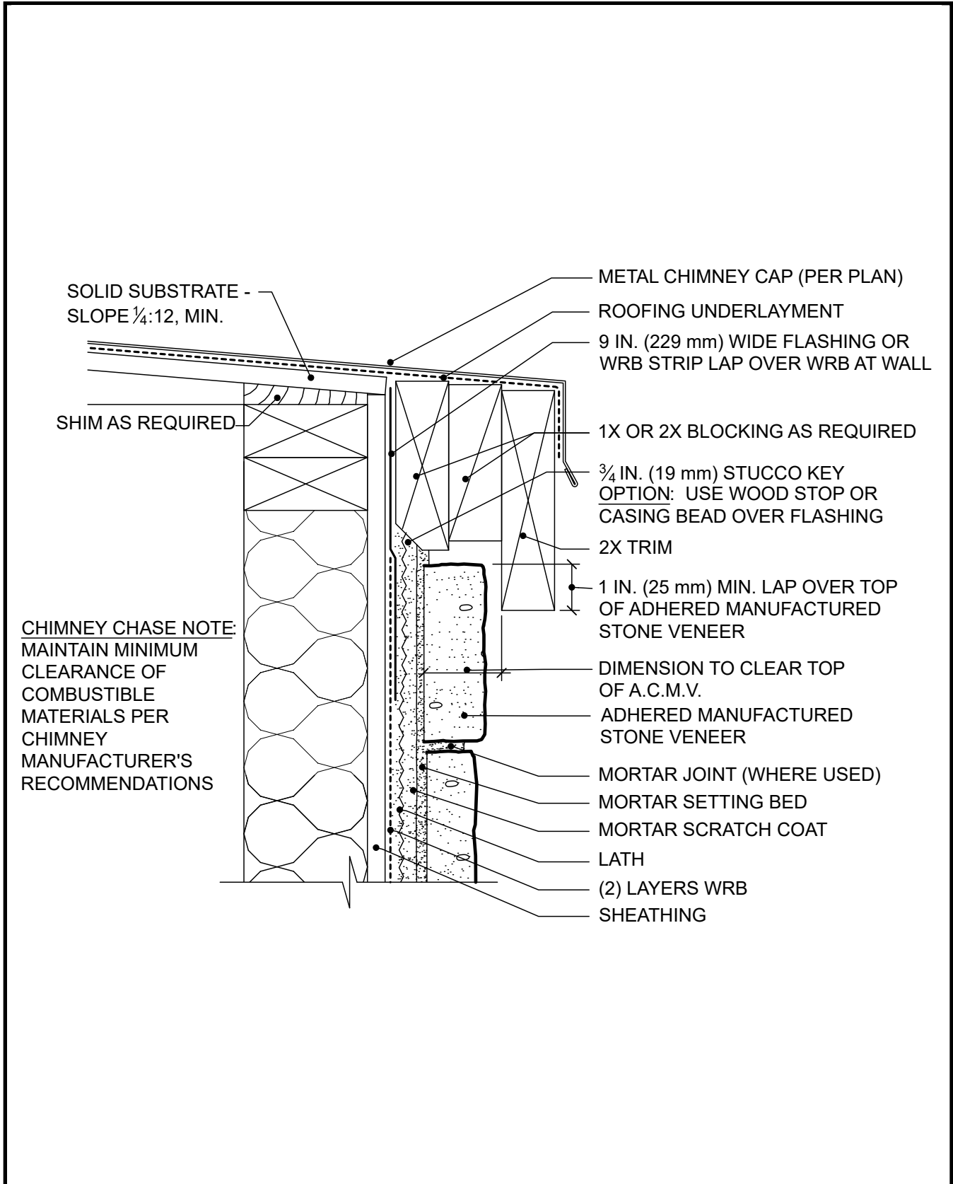
Figure 26. Chimney Chase
