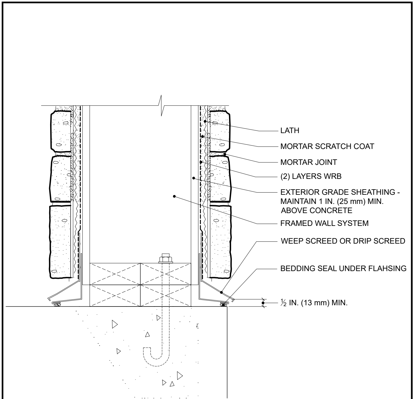
Figure 27. Column Base
