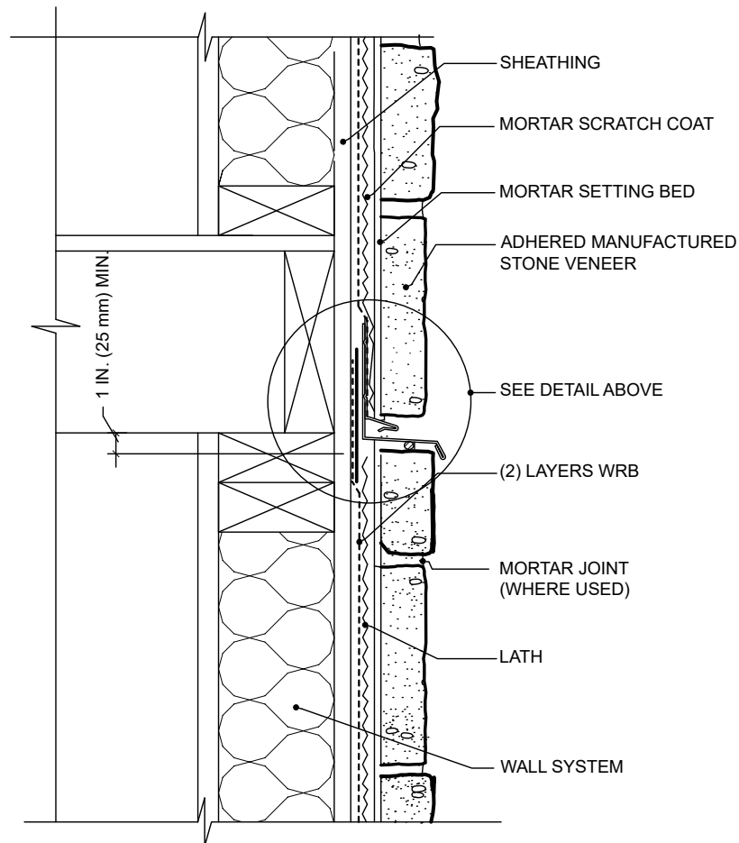
DETAIL
