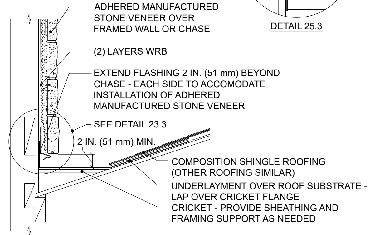
DETAIL 25.1
